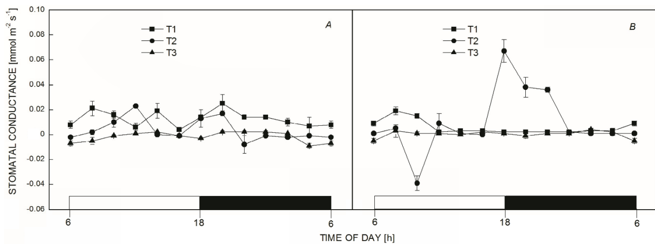
Fig. 4S. Stomatal conductance by Dendrobium nobile 'V4' (A) and Dendrobium chrysotoxum (B) in well-watered conditions (T1), 21 days without water (T2), and 28 days without water (T3), respectively. The results represent the means where n = 6 . Open bars represent light periods, closed bars represent dark periods.
