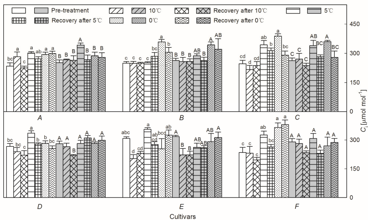
Fig. 4. Intercellular CO 2 concentration ( C_i ) of six rubber tree cultivars (A: Lan 873, B: Yunyan 77-2, C: Yunyan 77-4, D: GT1, E: Reken 523, and F: Reyan 733-97) before and after night-chilling treatment at 0, 5 or 10°C and subsequent recovery in full irradiance and 50% of full irradiance. Different letters indicate significant differences among groups in full irradiance (white bars) and 50% of full irradiance (gray bars) at P < 0.05 .
