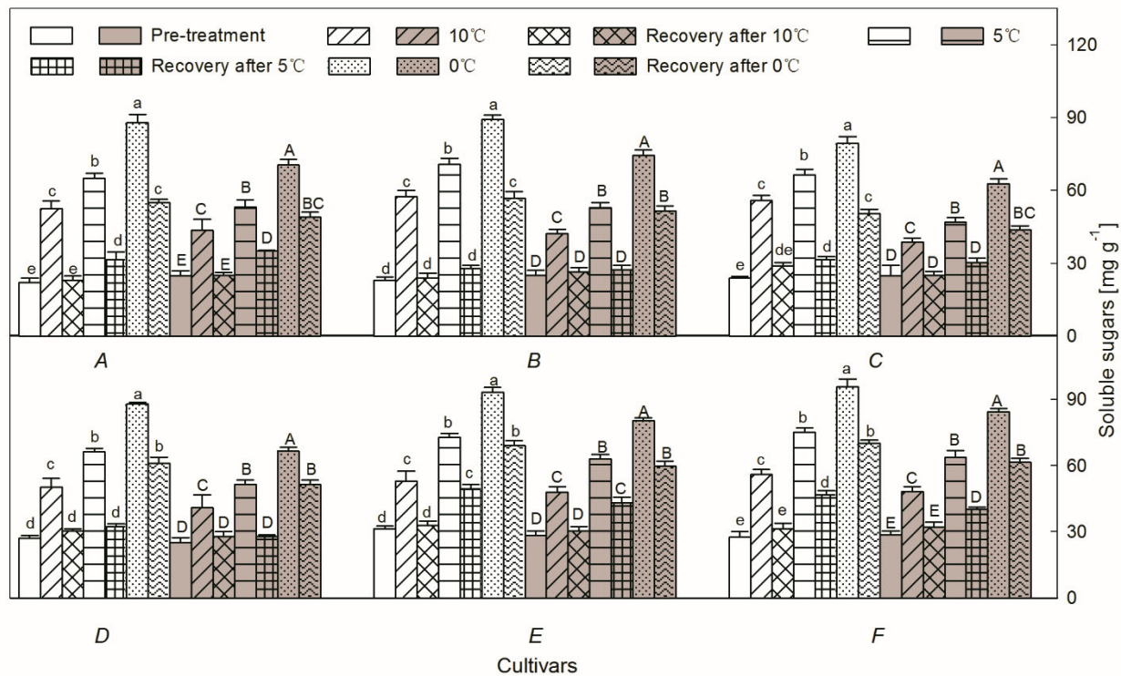
Fig. 7S. Soluble sugar content of six rubber tree cultivars (A: Lan 873, B: Yunyan 77-2, C: Yunyan 77-4, D: GT1, E: Reken 523, and F: Reyan 733-97) before and after night-chilling treatment at 0, 5 or 10°C and subsequent recovery in full irradiance and 50% of full irradiance. Different letters indicate significant differences among groups in full irradiance (white bars) and 50% of full irradiance (gray bars) at P < 0.05 .
