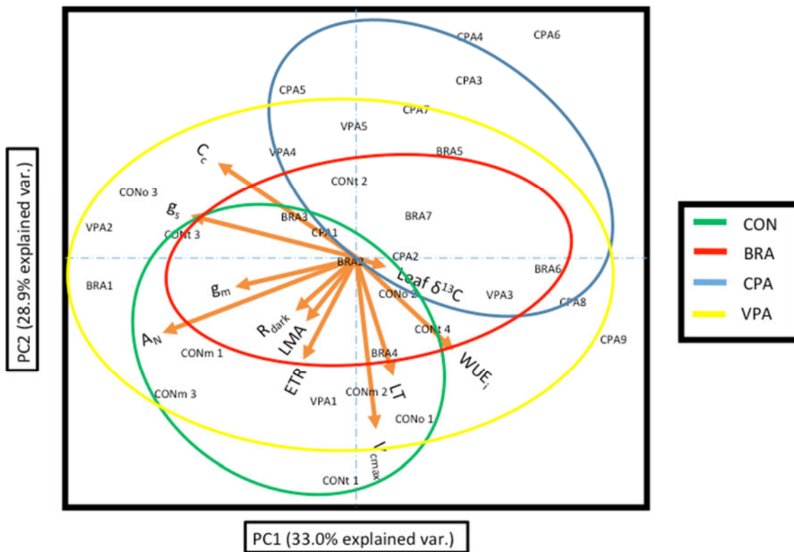
Fig. 1S. Principal component analysis of eleven photosynthetic and leaf morphological parameters for all the accessions. Accessions and group labels as Table 1.
