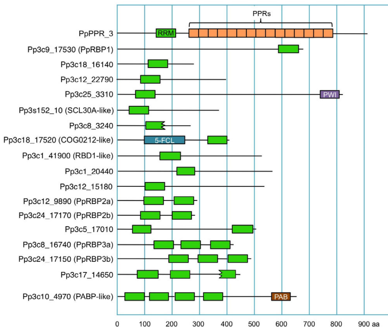
Supplementary Fig. 1. Schematic diagrams showing the domain structure of PpPPR_3 and newly identified chloroplastic RRM proteins.
