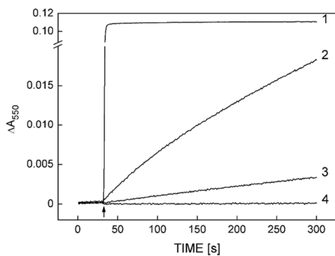
Fig. 2S. Kinetics of cytochrome c reduction by 1 mM ferrocyanide (1), 1 mM DPC (2), 1 mM \text{NH}_2\text{OH} (3), and 1 mM \text{MnCl}_2 . Cyt c^{\text{ox}} was dissolved in the buffer medium containing 50 mM MES-NaOH (pH 6.5) and 35 mM NaCl. Up arrow indicates an injection of the chemicals.
