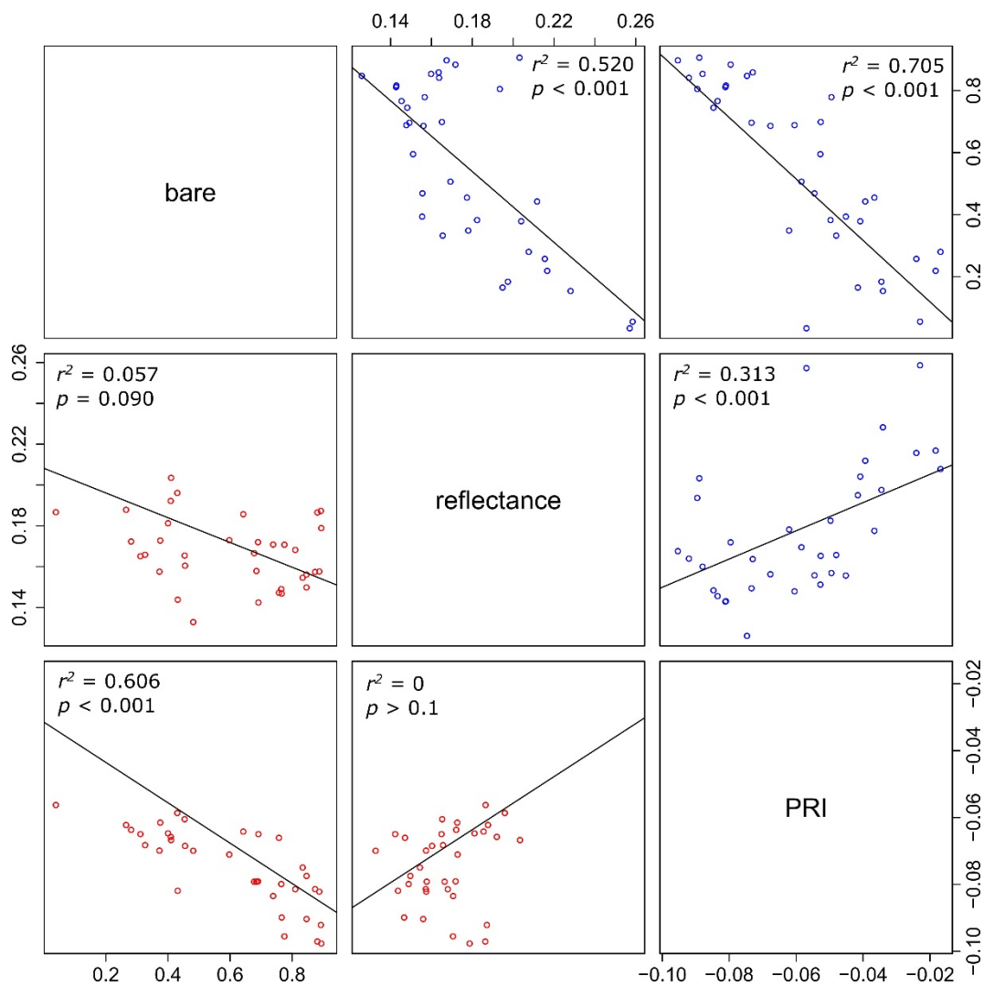
Fig. 1S. Pairwise scatterplots of bare ground percentage, mean reflectance, and PRI across plots in June ( upper right triangle ) and August ( lower left triangle ), with least-squares best fit lines.
