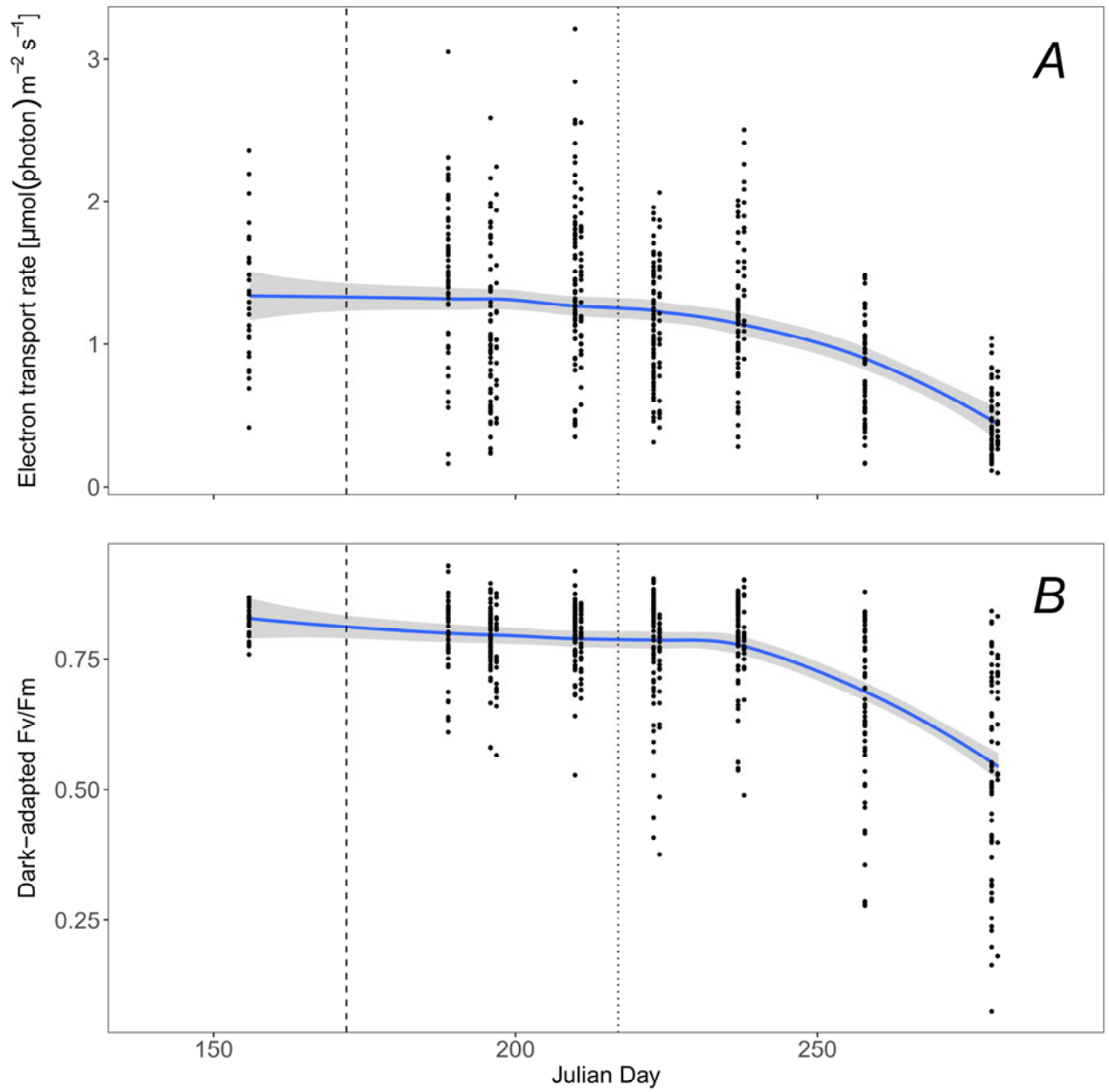
Fig. 2S. Seasonal change in (A) ETR and (B) dark-adapted F_v/F_m with LOESS fits (span = 0.75). Dashed and dotted lines are as in Figs. 1 and 2.
