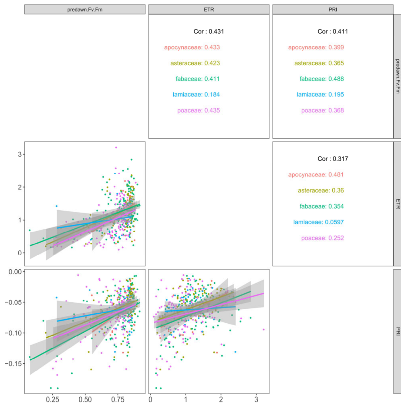
Fig. 3S. Pairwise correlations between ETR, F_v/F_m , and PRI across families, with least-squares best-fit lines.
