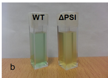
Fig. 1S. (a) Whole-cell absorption measured in Synechocystis \Delta PSI cells (orange) and WT cells (green). The spectra have been normalized relative to the 623 nm peak corresponding to phycocyanin absorption. (b) Cuvettes containing the samples.
