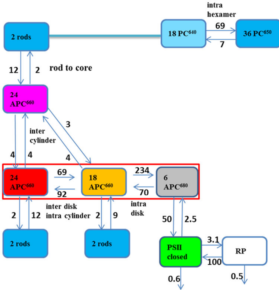
Fig. 2S. Functional compartmental model of the PB-PSII complex with RCs closed at RT, with a zoom out of a rod consisting of three lumped hexamers in the upper right. All microscopic rate constants are in 1/ns. The common k_{\eta} rate constant for excited PC and APC states of 0.78/ns has been omitted for clarity.
