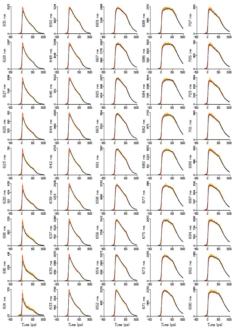
Fig. 3S. Emission at 45 wavelengths (indicated in the ordinate label) after 590 nm excitation at RT. Key: TR4 (grey), TR2 (orange). Black and red lines indicate the simultaneous target analysis fit. Note that the time axis is linear until 150 ps and logarithmic thereafter. Note also that each panel is scaled to its maximum. Overall rms error of the fit was 10.52.
