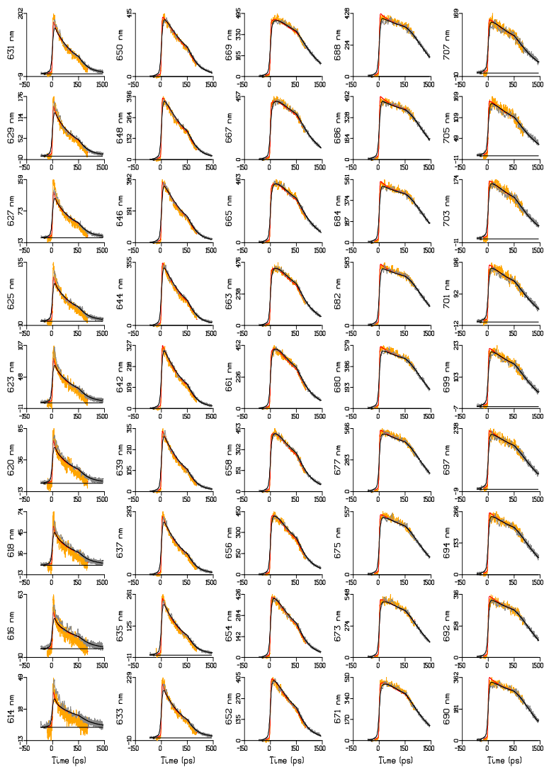
Fig. 4S. Emission at 45 wavelengths (indicated in the ordinate label) after 400 nm excitation at RT. Key: TR4 (grey), TR2 (orange). Black and red lines indicate the simultaneous target analysis fit. Note that the time axis is linear until 150 ps and logarithmic thereafter. Note also that each panel is scaled to its maximum. Overall rms error of the fit was 4.32.
