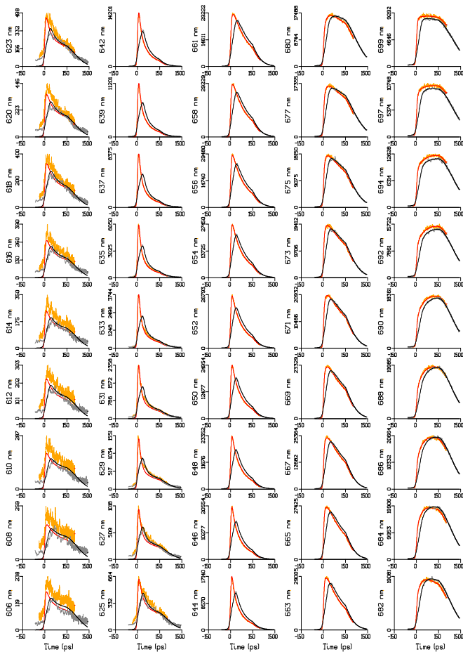
Fig. 6S. Emission at 45 wavelengths (indicated in the ordinate label) after 590 nm excitation at 77K. Key: TR4 (grey), TR2 (orange). Black and red lines indicate the simultaneous target analysis fit. Note that the time axis is linear until 150 ps and logarithmic thereafter. Note also that each panel is scaled to its maximum. Overall rms error of the fit was 62.
