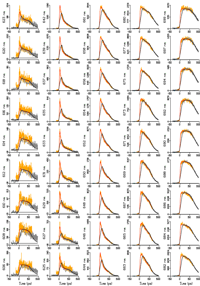
Fig. 7S. Emission at 45 wavelengths (indicated in the ordinate label) after 400 nm excitation at 77K. Key: TR4 (grey), TR2 (orange). Black and red lines indicate the simultaneous target analysis fit. Note that the time axis is linear until 150 ps and logarithmic thereafter. Note also that each panel is scaled to its maximum. Overall rms error of the fit was 18.7.
