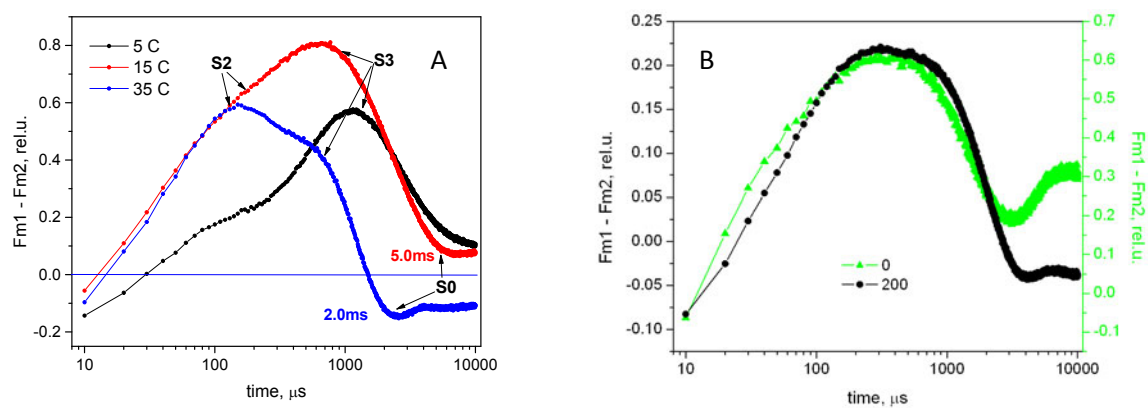
Fig. 3S. (A) S-state transition times in A. maxima in the presence of 1 M DIC at 5, 15, and 35°C. (B) Fluorescence curves from Figure 5A overlaid at different scales to demonstrate differences in S-state transition times.
