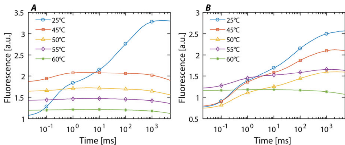
Fig. 1S. Fast chlorophyll fluorescence induction transients measured at room temperature from dark-adapted thylakoid membranes after 5-min incubation at different temperatures. (A) in control buffer; (B) in buffer with additional 2 M sucrose.
