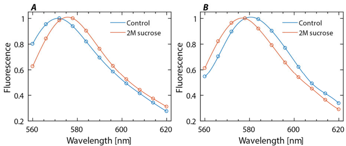
Fig. 2S. Stationary fluorescence emission spectra of MC540 ( A ) 10 \mu M MC540 in control buffer and in buffer with additional 2 M sucrose ( B ) thylakoid membranes resuspended in control buffer + 10 \mu M MC540, and in buffer with additional 2 M sucrose.
