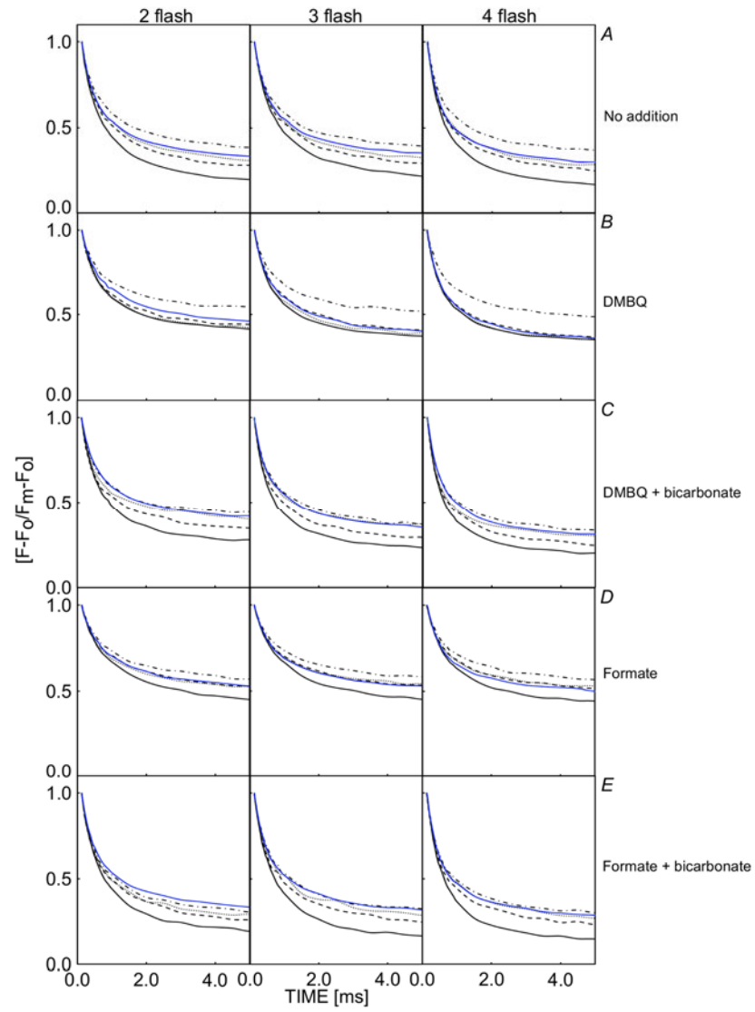
Fig. 4S. Chlorophyll a fluorescence relaxation for the first 5 ms, after being exposed to two, three and four actinic flashes given at 5 Hz. Wild type (black line); \Delta\text{PsbM} (dots); \Delta\text{PsbY} (dashes); \Delta\text{PsbM}:\Delta\text{PsbY} (dashes and dots) and Y_{\text{comp}} (blue line). Data are the average of three biological replicates.
