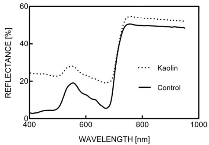
Fig. 2S. Typical grapevines spectral reflectance for leaves with (dashed line) and with no kaolin (control, solid line ) ( n = 8 ).
