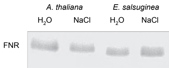
Fig. 1S. Changes in the amount of ferredoxin:NADP + oxidoreductase (FNR) in A.thaliana and E. salsuginea plants irrigated with water and with NaCl solution. Salinity of 0.15 and 0.3 M, was used for A. thaliana and E. salsuginea , respectively. Immunoblotting was done with leaf extracts of soluble proteins, for visualization 5 µg protein per lane was loaded.
