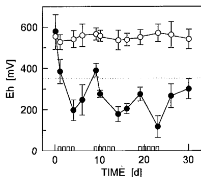
Fig. 1. Changes in soil redox potential (Eh) conditions for two soil treatments (○ - control, ● - intermittently flooded, □ - flooding days) during the experiment. An Eh value of +350 mV represents the value at which oxygen disappears from the soil. Vertical lines represent SE. Vertical bars represent days flooded for the intermittently flooded treatment ( n = 6 ).
