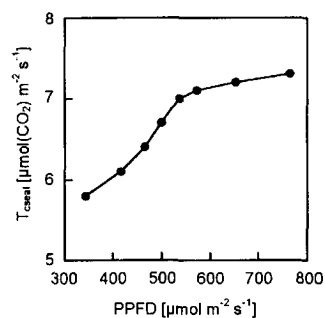
Fig. 3. Change in T_{cseal} with irradiance (PPFD) at leaf temperature of 30 °C. T_{cseal} was calculated by the Eq. (6).
