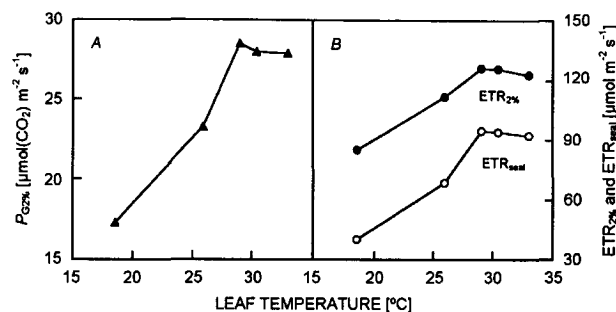
Fig. 4. Changes in P_{G2\%} , ETR_{2\%} , and ETR_{seal} with leaf temperature at an irradiance of 500 \mu\text{mol m}^{-2} \text{s}^{-1} .
