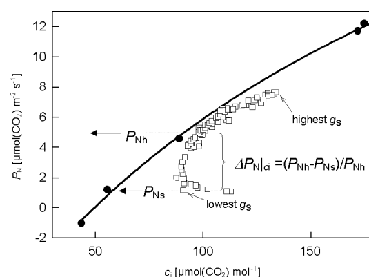
Fig. 4. The \text{CO}_2 response of photosynthesis of a single sunflower leaf before ABA treatment (solid circles and line) and after 10 d of plant feeding with 10^{-5} \text{ M} ABA in nutrient solution (open squares). Parameters of the hyperbolic regression curve are: V_{\text{cmax}} = 40.2 \mu\text{mol}(\text{CO}_2) \text{ m}^{-2} \text{ s}^{-1} , \Gamma = 49.3 \mu\text{mol}(\text{CO}_2) \text{ mol}^{-1} , O = 245 \mu\text{mol}(\text{CO}_2) \text{ mol}^{-1} (see Eq. A1 in Appendix for further explanation). The variation of c_i (and g_s ) in the ABA affected leaf was obtained during oscillations of gas exchange parameters shown in Fig. 6A,B. Ambient \text{CO}_2 concentration was 180 \mu\text{mol}(\text{CO}_2) \text{ mol}^{-1} . Calculation of photosynthesis depression at a particular c_i ( \Delta P_{N|c_i} ) is shown.
