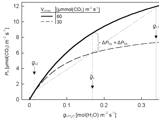
Fig. 1. A diagram showing how the photosynthetic rate P_N of a non-stressed leaf having uniform stomatal conductance \bar{g}_s drops by the \Delta P_{\text{Np}} value in a patchy leaf when one half of stomata population closes ( g_{s2} ) and the other half opens to ( g_{s1} ) so that \bar{g}_s remains unchanged. The new rate of photosynthesis affected by patchiness is then an arithmetic mean of P_N at g_{s1} and P_N at g_{s2} (Terashima et al. 1988, Farquhar 1989). The P_N(g_s) relation of the non-stressed leaf with carboxylation capacity V_{\text{cmax}} = 60 \mu\text{mol}(\text{CO}_2) \text{ m}^{-2} \text{ s}^{-1} is represented by the solid curve; the dashed curve shows the P_N response to g_s when V_{\text{cmax}} is one half of its value in the non-stressed leaf. If g_s is uniformly distributed and has the \bar{g}_s value, then the biochemical depression of photosynthesis \Delta P_{\text{Nb}} equals \Delta P_{\text{Np}} . The curves were calculated using Eq. A3 (Appendix) where O = 245 \mu\text{mol}(\text{CO}_2) \text{ mol}^{-1} , c_a = 180 \mu\text{mol}(\text{CO}_2) \text{ mol}^{-1} , and \Gamma = 50 \mu\text{mol}(\text{CO}_2) \text{ mol}^{-1} and g_s varied between 0 and 0.22 \text{ mol}(\text{CO}_2) \text{ m}^{-2} \text{ s}^{-1} (see Eq. A1 in Appendix). The results are plotted versus g_s in \text{mol}(\text{H}_2\text{O}) \text{ m}^{-2} \text{ s}^{-1} .
