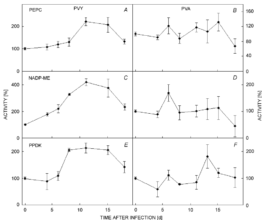
Fig. 4. Activities of PEPC, NADP-ME, and PPDK from tobacco leaves of cv. Samsun 4–18 d after inoculation by PVY (A, C, E) or by PVA (B, D, F) calculated per fresh mass. The activity of each sample is calculated as percentage of the non-infected control, where 100 % of PEPC is 1.40 \pm 0.17 \mu\text{mol s}^{-1} \text{kg}^{-1} (A, B), 0.50 \pm 0.08 \mu\text{mol s}^{-1} \text{kg}^{-1} of NADP-ME (C, D) and 0.58 \pm 0.01 \mu\text{mol s}^{-1} \text{kg}^{-1} of PPDK (E, F). Means \pm S.E. In each repetition of the experiment, the activity was measured in triplicate.
