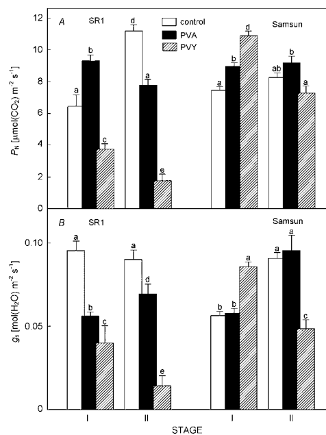
Fig. 2. Net photosynthetic rate ( P_N ; A) and stomatal conductance ( g_s ; B) of tobacco cv. Samsun and SR1 infected by PVY or PVA at two different stages of infection. Stage I, i.e. first visible symptoms of virosis appear on the leaves (about 5 d after inoculation by PVY and 7 d after inoculation by PVA). Stage II (about 15 d after inoculation by PVY and 18 d after inoculation by PVA). Means \pm S.E. Different lower-case letters mark statistically significant differences at p = 0.05 .
