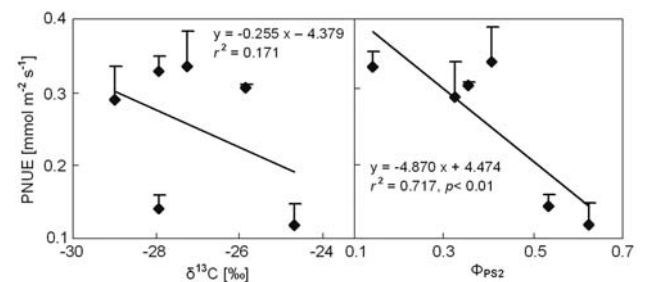
Fig. 2. Relationships of leaf stable carbon isotope composition ( \delta^{13}C ) and actual quantum yield of PS2 electron transport ( \Phi_{PS2} ) with photosynthetic nitrogen use efficiency (PNUE) in the six tree seedlings. Error bars are \pm SE , n = 3 .
