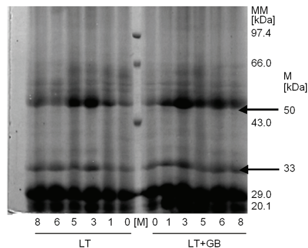
Fig. 4. Effects of glycine betaine (GB) on thylakoid polypeptides of tobacco leaves. The numbers 0, 1, 3, 5, 6, and 8 represent the treatment and recovery days; MM is molecular mass, M represents molecular mass markers.
