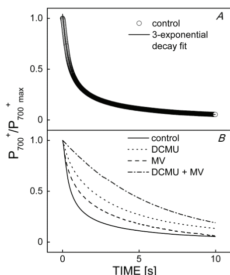
Fig. 5. Rereduction kinetics of P 700 absorbance following cessation of illumination with FR light. (A) a three-exponential decay fit for the average of control traces and (B) average traces measured in control leaf disks and disks infiltrated with 200 \mu M 3-(3,4-dichlorophenyl)-1,1-dimethylurea (DCMU), 600 \mu M methyl viologen (MV), or both (DCMU + MV) ( n \geq 4 ). Leaf disks were taken from plants grown as described in Fig 1.
