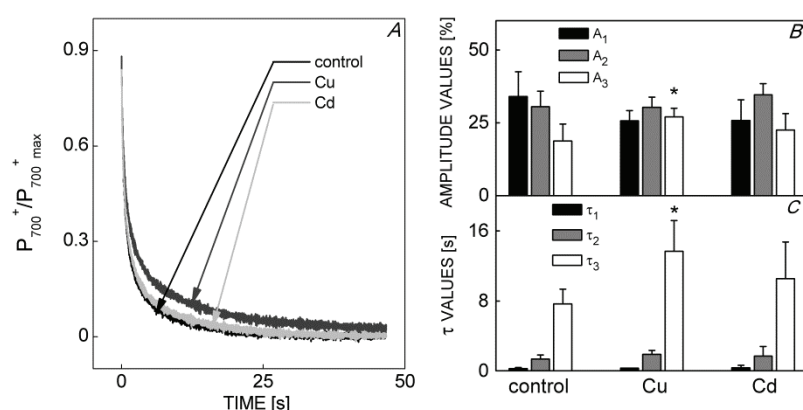
Fig. 6. Rereduction kinetics of P 700 absorbance measured in leaf disks from plants grown as described in Fig 1. (A) average traces. The amplitude values – A_1 , A_2 , and A_3 (B), and time constants – \tau_1 , \tau_2 and \tau_3 (C) – were obtained by fitting traces with three exponential components. (The numbers 1, 2 and 3 in subscript indicate fast, middle, and slow phases). Bars represent means \pm SD ( n \geq 6 ). Asterisks indicate the level of significance by Student t -test: * – P < 0.05 .
