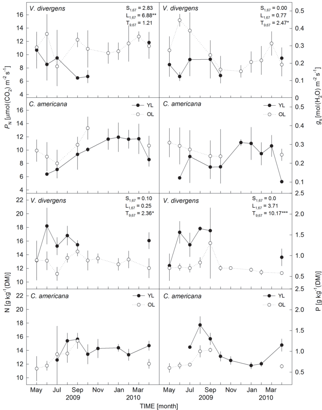
Fig. 5. Area-based leaf photosynthesis (left top panels), stomatal conductance (right top panels), leaf nitrogen (left bottom panels) and phosphorus (right bottom panels) concentration for young (YL, solid circles, solid lines) and old (OL, open circles, dotted lines) leaves of V. divergens (top panels) and C. americana (bottom panels) during the May 2009–April 2010 study period. Also shown are the results of a 3-way ANOVA ( F -statistics and degrees of freedom) for the effects of species (S), leaf age (L) and season (T). Mean \pm SE ( n = 5 ). * p < 0.05 ; ** p < 0.01 ; *** p < 0.001 .
