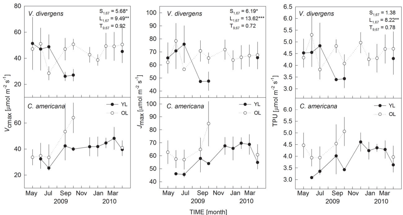
Fig. 6. Area-based maximum rate of carboxylation (left panels), electron transport (middle panels) and triphosphate utilization (right panels) for young (YL, solid circles, solid lines) and old (OL, open circles, dotted lines) leaves of V. divergens (top panels) and C. americana (bottom panels) during the May 2009–April 2010 study period. The results of a 3-way ANOVA ( F -statistics and degrees of freedom) for the main effects of species (S), leaf age (L) and season (T) are also shown. Mean \pm SE ( n = 5 ). ^*p < 0.05 ; ^{**}p < 0.01 ; ^{***}p < 0.001 .
