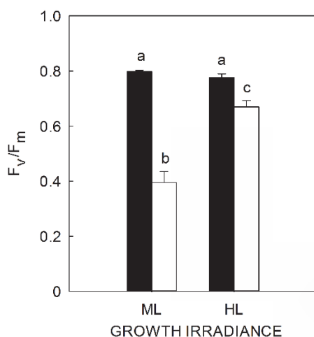
Fig. 2. Photoinhibition of photosynthesis in leaves of Eutrema (Yukon ecotype) developed at different growth irradiance. Plants were grown under either 250 (ML) or 750 \mu\text{mol}(\text{photon})\text{ m}^{-2}\text{ s}^{-1} (HL) PPFD. Responses were determined by monitoring changes in the F_v/F_m ratio prior photoinhibition (black bars) and post photoinhibition (white bars). Values represent means \pm SD ( n = 8 ). Bars with different letters are significantly different at P=0.05 based on a one-way ANOVA. F_v/F_m – maximal quantum yield of PSII photochemistry; HL – high light; ML – moderate light.
