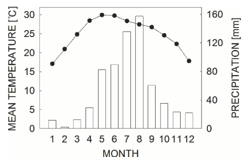
Fig. 1. Monthly mean air temperature (black circles) and monthly precipitation (vertical bars) in the study site. The values are the means of 2012 to 2014.
