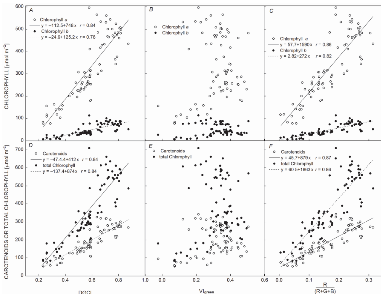
Fig. 5. Relationships between chlorophyll and carotenoids contents measured analytically in laboratory and the image based on DGCI index (A,D), VI_{\text{green}} (B,E), and NRI (C,F) in the leaves of the soybean.
