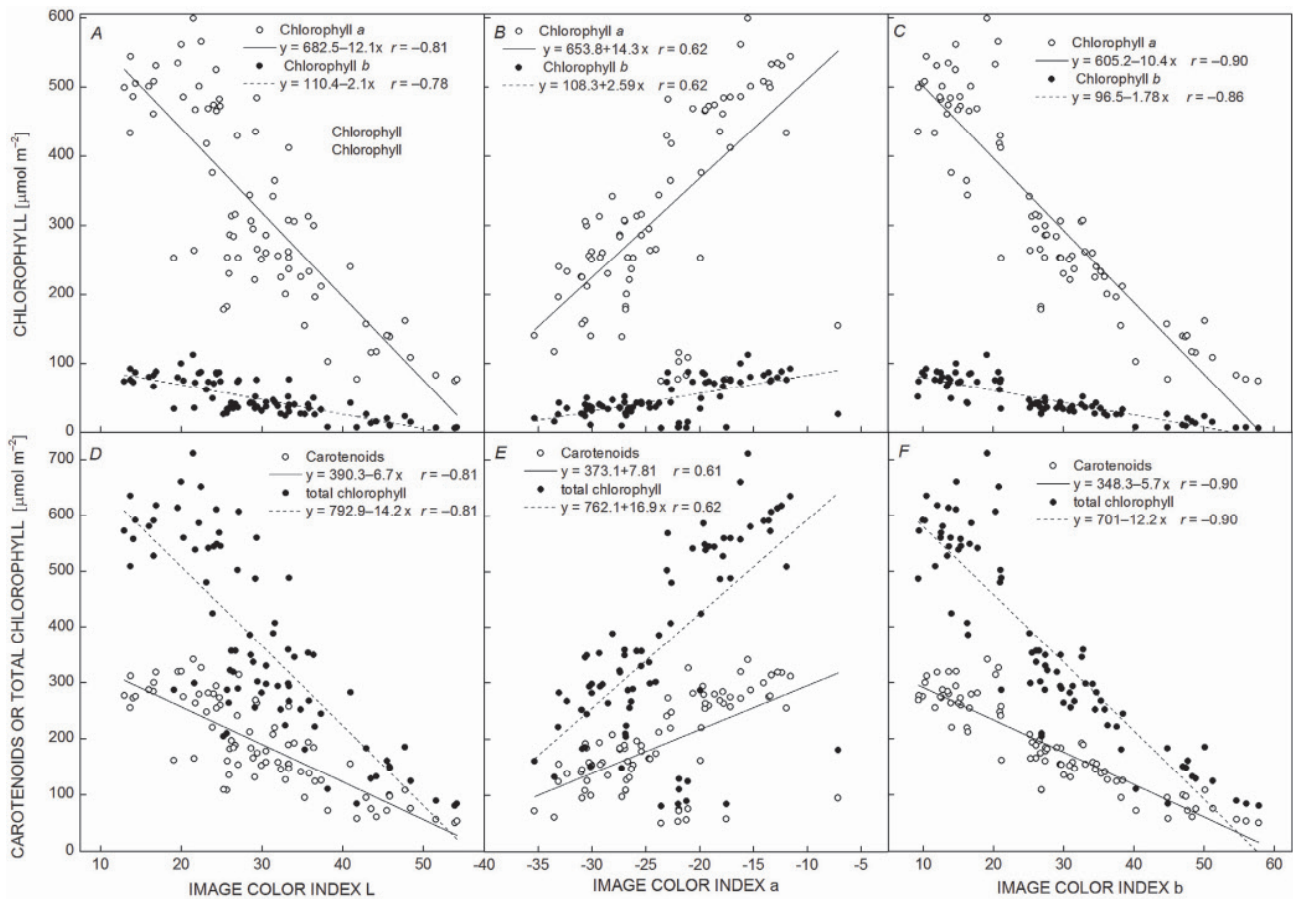
Fig. 3. Relationships between chlorophyll and Car content measured analytically in the lab and from an image based on the CIE L^*a^*b color model with indices L (A,D), a (B,E), and b (C,F) in soybean leaves.
