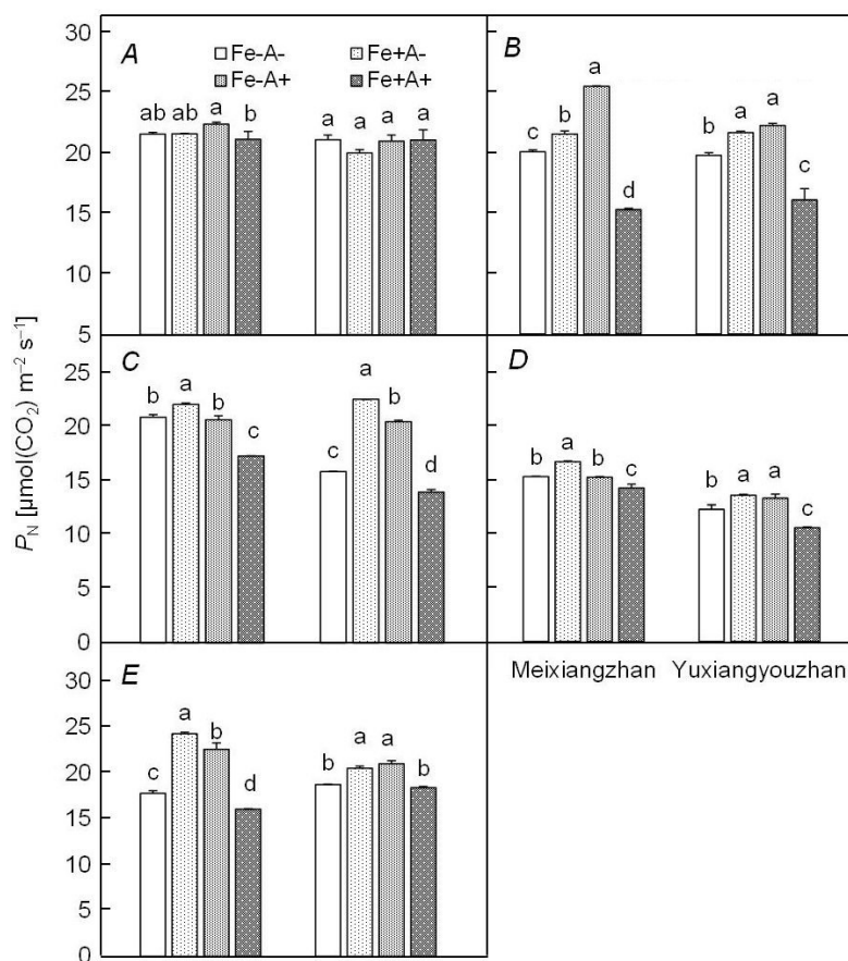
Fig. 1. Effect of Fe and \alpha -ketoglutaric acid on the net photosynthetic rate ( P_N ) at (A) 1 DAS, (B) 2 DAS, (C) 3 DAS, (D) 4 DAS, and (E) 5 DAS for Meixiangzhan and Yuxiangyouzhan. Vertical bars with different lowercase letters above are significantly different at P < 0.05 by LSD tests. Capped bars represent SD ( n = 3 ). Fe-: 0 mg( \text{FeCl}_3 ) \text{kg}^{-1} ; Fe+: 20 mg( \text{FeCl}_3 ) \text{kg}^{-1} ; A-: 0 mg( \alpha -ketoglutaric acid) \text{L}^{-1} ; A+: 50 mg( \alpha -ketoglutaric acid) \text{L}^{-1} . DAS – days after spraying.
