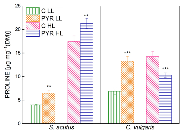
Fig. 3. Effects of different light intensities on the proline content of Scenedesmus acutus and Chlorella vulgaris with PYR exposure. Error bars represent standard deviation ( n = 3 ). *** ( p < 0.001 ), ** ( p < 0.01 ), and * ( p < 0.05 ) represent significant differences between the control and treatments, ns = nonsignificant. C – control; HL – high light; LL – low light; PYR – pyrene.
