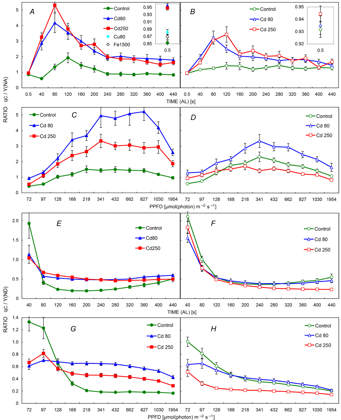
Fig. 8. The ratios showing balance of limitations between the acceptor side of PSII ( q_C ) and the acceptor [ Y_{(NA)} ] or donor [ Y_{(ND)} ] sides of PSI. (A–D) ratios q_C / Y_{(NA)} ; (E–H) ratios q_C / Y_{(ND)} . (A, B, E, F) Induction curves (IC); (C, D, G, H) rapid light curves (RLC). All other designations are the same as in Figs. 2 and 7.
