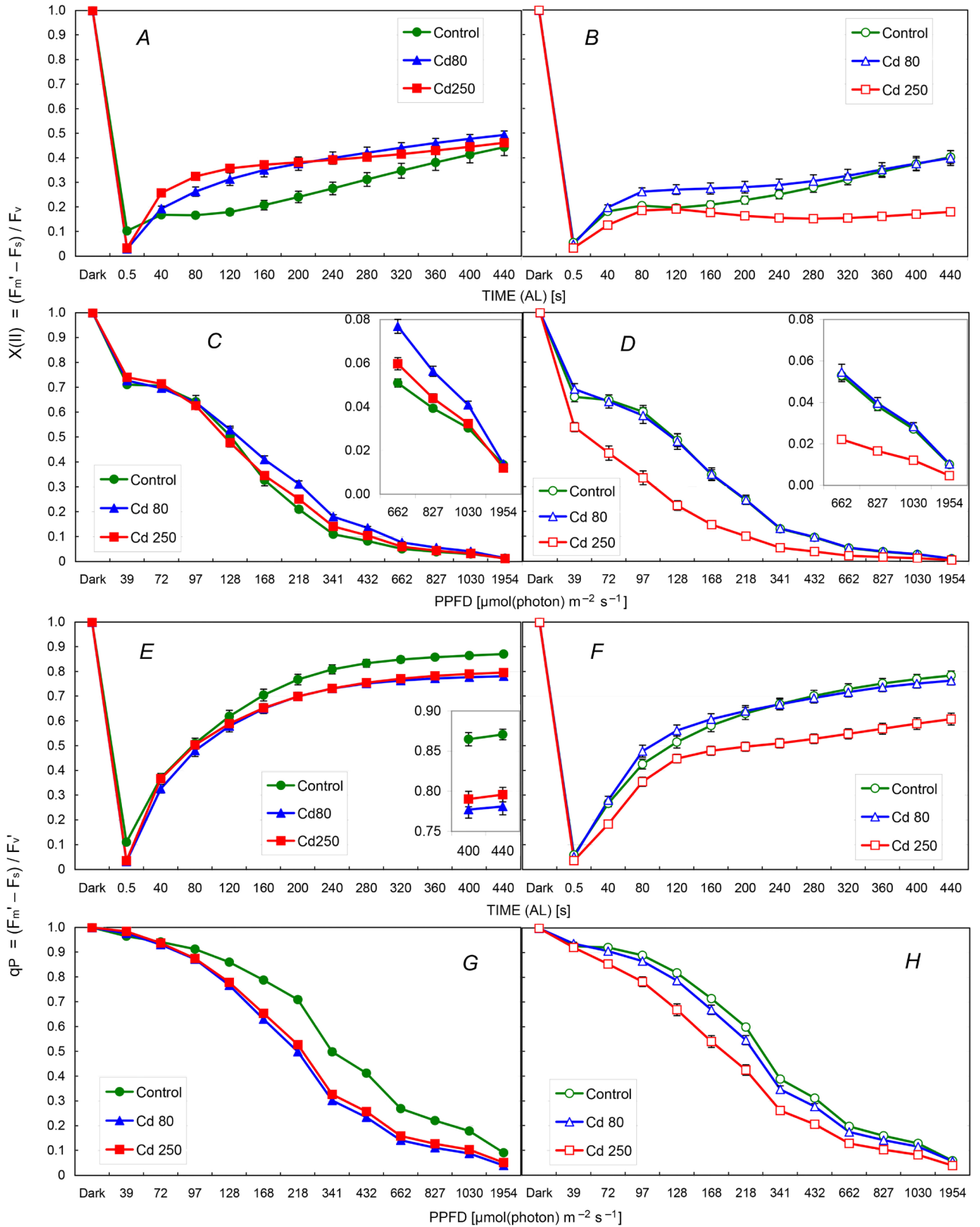
Fig. 2. Dynamics of photochemical coefficients X_{(II)} and q_P of PSII. (A–D) X_{(II)} ; (E–H) q_P (dynamics of \Phi_{PSII} are represented in Fig. 2S). (A,B,E,F) Induction curves (IC); (C,D,G,H) rapid light curves (RLC). Lines represent the variants of treatment: green circles – control, blue triangles – Cd 80 \mu\text{M} , red squares – Cd 250 \mu\text{M} . Filled symbols represent barley; open symbols represent maize. AL – actinic light. Data are presented as means \pm SE. The insets show the corresponding values with the higher resolution.
