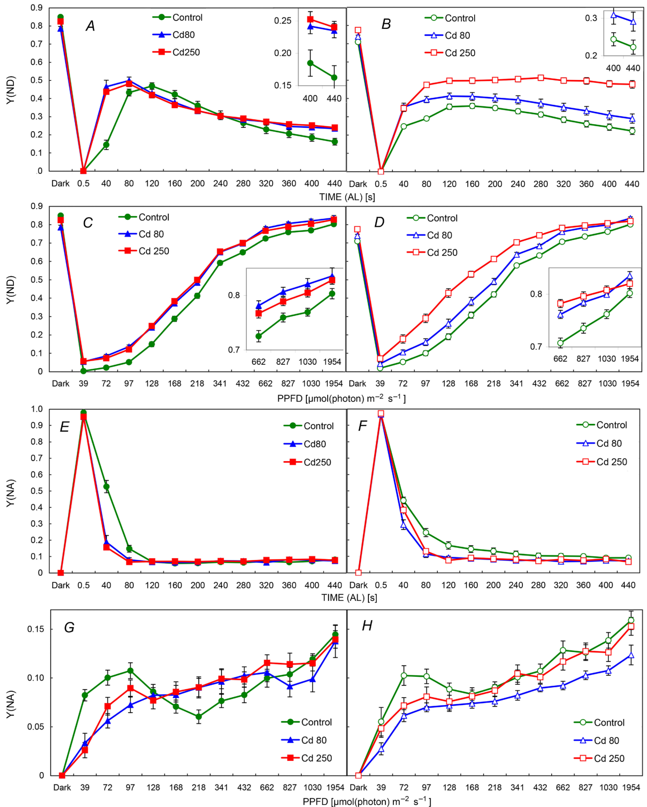
Fig. 6. Dynamics of the limitations of PSI. (A–D) limitation at the donor side, Y(ND) ; (E–H) limitation at the acceptor side, Y(NA) . (A,B,E,F) Induction curves (IC); (C,D,G,H) rapid light curves (RLC). All other designations are the same as in Fig. 2.
